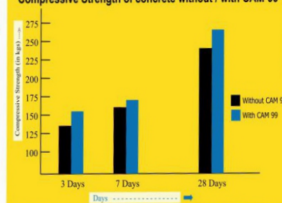
Compressive Strength of concrete without / with CAM-99
